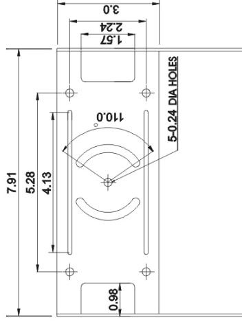
MONITOR MOUNTING HOLE PATTERN
